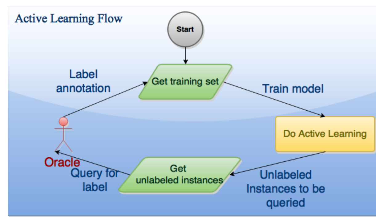
Figure 3: Active learning flow [1]
