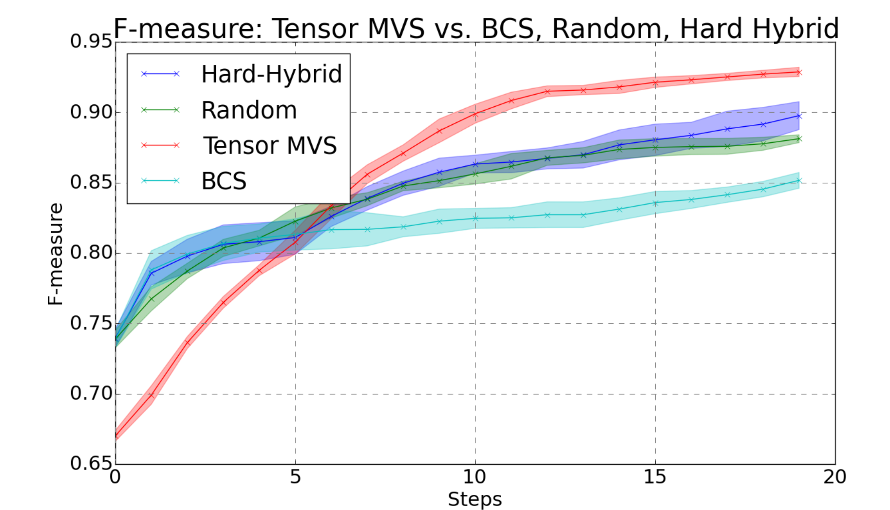
Figure 2: Comparison of the results of Tensor MVS method using speaker modality and speaker annotation for 20 steps
