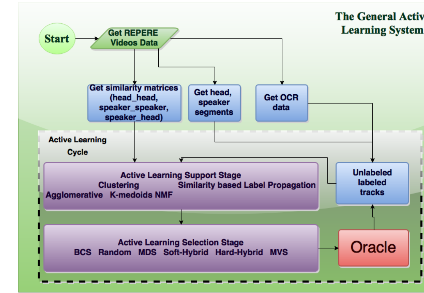
Figure 1: Active learning flow [1]
